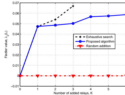
Fig. 6. The Fiedler value versus the number of added relay for a disconnected sensor network consisting of n = 200 nodes and deployed in a 25 \times 25 area.
