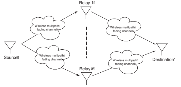
Fig. 1. Simplified system model for the distributed space-frequency codes.
